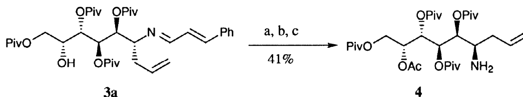
Scheme 3: a: Ac 2 O, pyridine; b: 1N HCl, 2,4-dinitrophenylhydrazine, MeOH, CH 2 Cl 2 , r.t.; c: NaHCO 3
