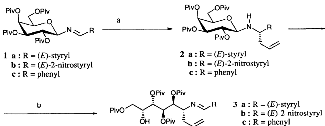
Scheme 1. a: Allyltrimethylsilane or allyltributylstannane, \text{SnCl}_4 , THF. Piv = (\text{CH}_3)_3\text{C-CO} ; b: 1.1 eq. Lewis acid (conditions see Table 1).
